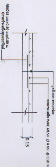
CONTRACTION JOINT
